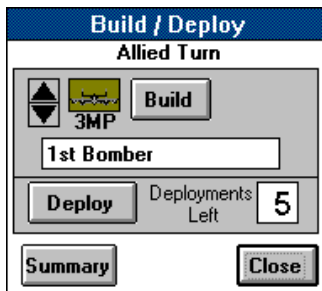
Exhibit 6- Build/Deploy Window
